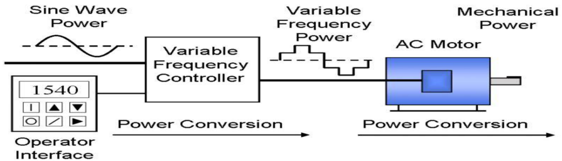
Fig 5: VFD system schematic
